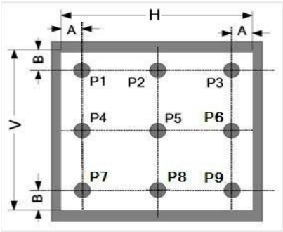
FIG. 1. Measuring method for Contrast ratio,surface luminance, Luminance uniformity,CIE (x, y) chromaticity对比度，表面亮度，均匀度，CIE坐标测试方法
