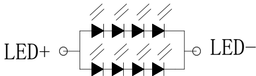
LED CIRCUIT DIAGRAM
