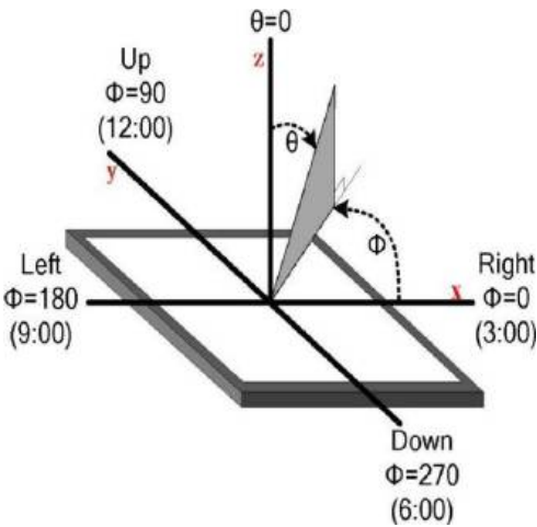
FIG.3. The definition of viewing angle 视角定义
